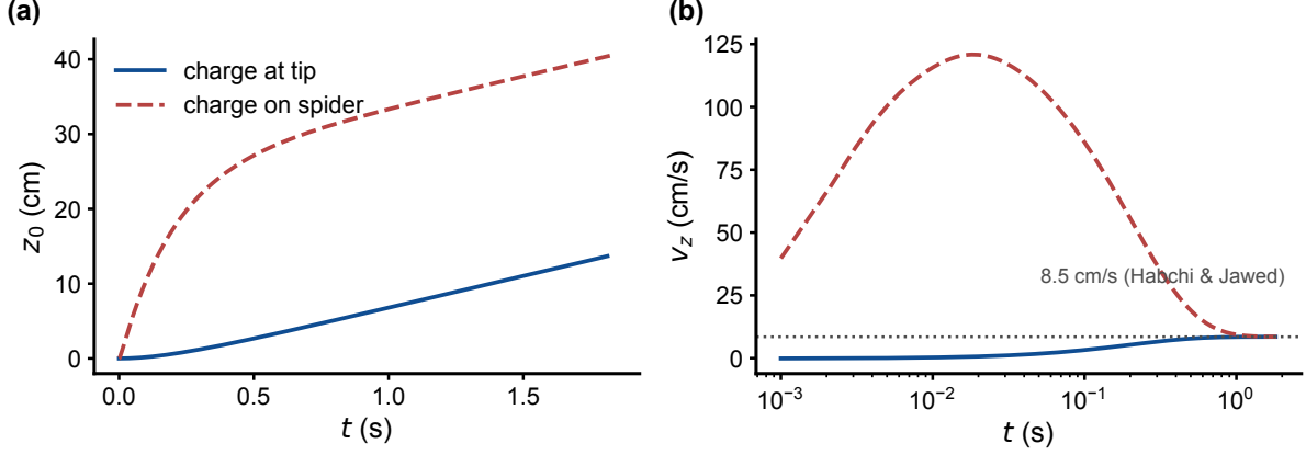
FIG. 2. Test 1: take-off of a spider ( m = 0.9 mg, Q_s = 0 ) with one thread ( L = 0.5 m, N_t = 100 ) in the chamber field of Eq. (2), with q = 1.2433 nC. (a) Altitude z_0(t) and (b) vertical velocity v_z(t) of the spider node, for the charge at the thread tip (solid) and on the spider node (dashed). The dotted line marks the steady velocity \approx 8.5 cm/s reported in [1]. With tip charge the velocity relaxes on the time scale t_s = m/(\eta_{\parallel}L + \zeta_s) = 0.20 s; with the charge on the spider, the enhanced field near the prominence ejects the spider at up to 1.21 m/s before it settles.
