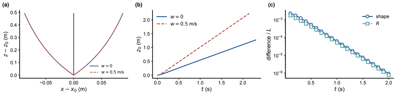
FIG. 9. Code test: shape invariance under a uniform updraft ( N = 4 , tip charge, q = 0.662 nC, \bar{F}_l = 2 , Q_s = 0 , constant E = 7.41 \times 10^3 V/m, N_t = 100 ). (a) Steady-state configurations in the frame of the spider for w = 0 (solid) and w = 0.5 m/s (dashed); the curves should coincide. (b) Ground-frame altitude z_0(t) ; the slopes differ by exactly w . (c) Both runs started at rest in the ground frame: maximum shape difference and tip-radius difference, normalized by L ; both decay exponentially with time constant 0.24 s.
