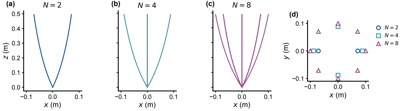
FIG. 5. Steady shapes of tip-charged bundles in still air ( L = 0.5 m, m = 1 mg, Q_s = 0 , \bar{F}_l = 2 , constant E = 7.41 \times 10^3 V/m, N_t = 100 ; parameters of Table VIII). (a)–(c) Side view of the threads in the frame of the spider for N = 2, 4 , and 8 . (d) Top view of the tips, which lie on a circle of radius R , as assumed in Sec. IV.
