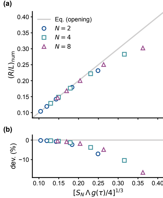
FIG. 3. Opening of the bundle. (a) Tip radius from simulation, (R/L)_{\text{num}} , versus the small-angle prediction of Eq. (31), for N = 2 (circles), 4 (squares), and 8 (triangles), and \bar{F}_l = 1.2, 1.5, 2, 3, 5 (tip charge, still air, m = 1 mg, Q_s = 0 , constant E = 7.41 \times 10^3 V/m). The solid line has slope 1. (b) Relative deviation from the prediction: below 1% for small openings, growing to about -17% at the largest opening ( N = 8 , \bar{F}_l = 5 ), which marks the breakdown of the small-angle approximation.
