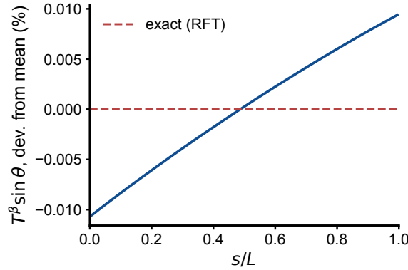
FIG. 4. Numerical check of the first integral of Eq. (22). The quantity T^\beta \sin \theta , normalized by its mean value, along one thread at steady state ( N = 2 , tip charge, q = 1.324 nC, \bar{F}_l = 2 , Q_s = 0 ), for N_t = 100 . Shown is the deviation from the mean in percent; the exact RFT result is zero (dashed line). The spread over the interior edges is 0.019%.
