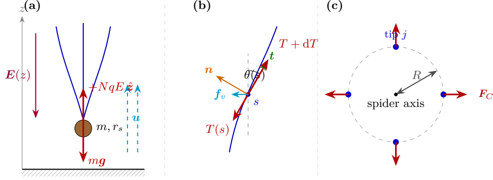
FIG. 1. (a) Schematic representation of the spider–silk system in atmospheric turbulence and a vertical electric field \mathbf{E}(z) . (b) Geometry and force equilibrium along a single flexible thread element at arc length s , showing local tangent \mathbf{t} , normal \mathbf{n} , angle \theta(s) , tension T(s) , and RFT drag \mathbf{f}_v . (c) Top view at s = L for N = 4 tip-charged threads, showing the conical opening of radius R driven by mutual radial Coulomb repulsion \mathbf{F}_C .
