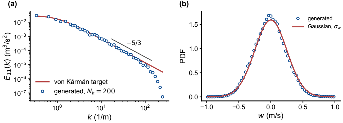
FIG. 6. Validation of the synthetic turbulence of Eq. (15), for \sigma_w = 0.25 m/s, \ell = 1 m, and N_k = 200 modes (average over 50 realizations). (a) Longitudinal one-dimensional spectrum of w along a vertical line versus the spectrum implied by Eq. (16); the generated spectrum is shown up to the resolution cut-off k_{\max} = 2\pi/(5\Delta l) and falls below the target in the last decade because of the finite shell width near k_{\max} . (b) Probability density of w with the Gaussian of standard deviation \sigma_w . [TO DO: Regenerate with the renormalized amplitudes of Stage B.]
